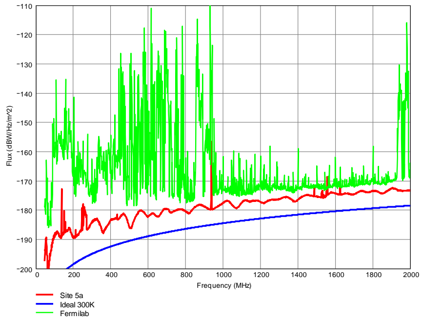
Figure 23. Comparison of RFI at Fermilab and Morocco Site 5a.
