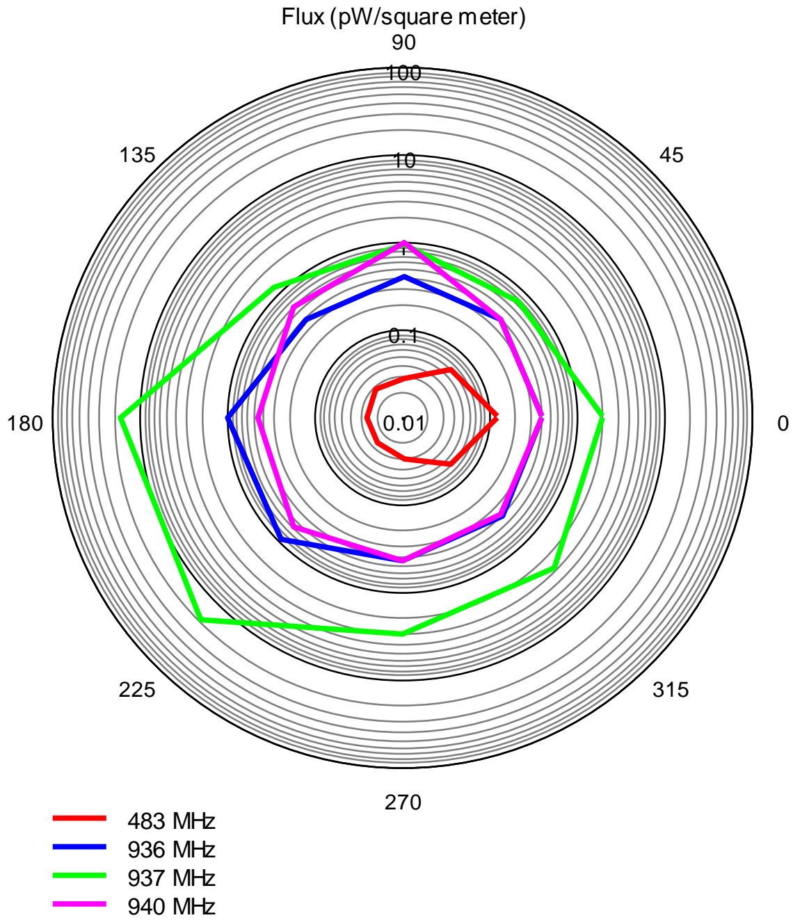
Figure 17. Directional plot of signal flux at Site 5a using the log-peridic antenna. The antenna has a beam width of about 60 degrees. The north direction is pointing up, the east direction is pointing to the right. The units of the plot is pW/m 2 .
